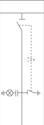
Cubicle with SF6 Insulated Disconnector
