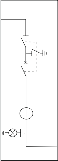
Single isolation Cubicle Lateral Outgoing (with Circuit Breaker and Sf6 insulated disconnector)
