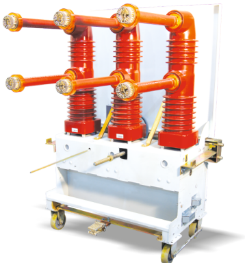
Circuit breaker on the truck
