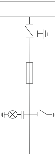
Cubicle with Fused Disconnector (with Air Rotary Disconnector) * for MME-24
